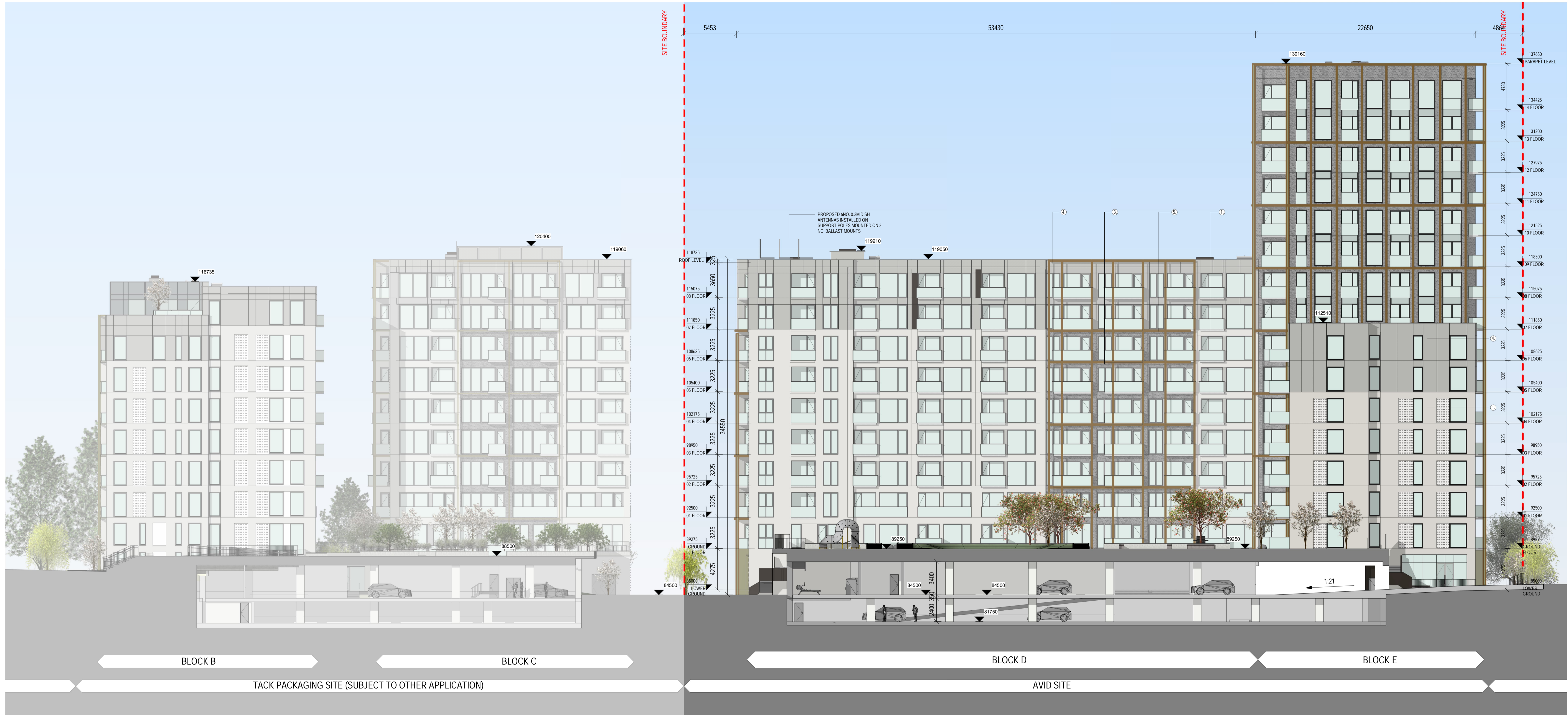
1 PROPOSED COURTYARD ELEVATION 01 - AVID SITE 1:200
